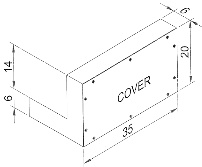
WIRE GUTTER # 3
