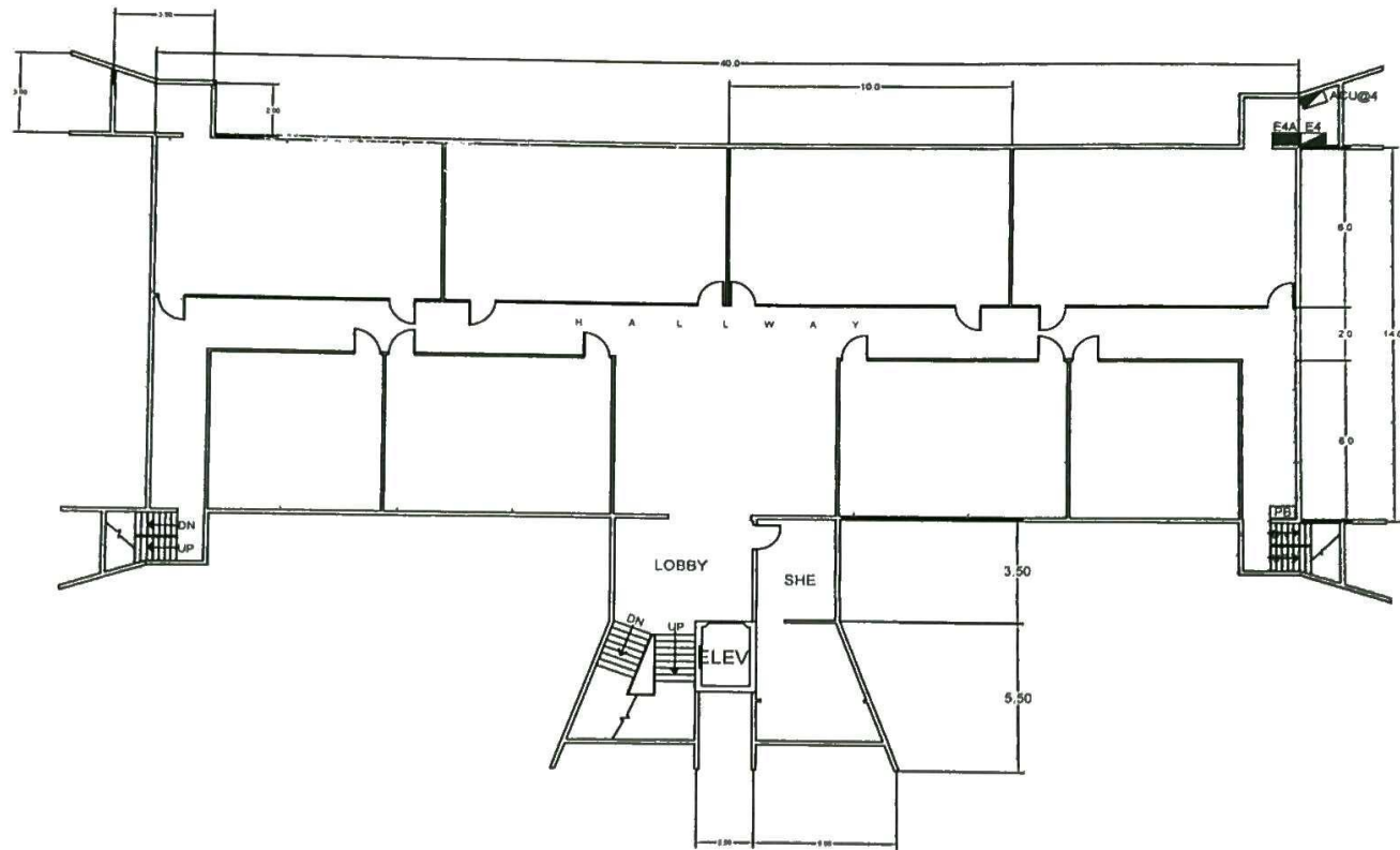
FOURTH FLOOR POWER LAYOUT (GUSALING LACSON) SCALE: 1:100 METERS
