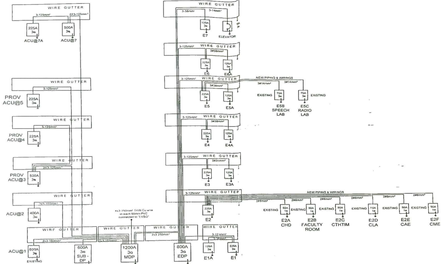
REMODELING OF ELECTRICAL RISER (GUSALING LACSON) ANY CONVENIENT SCALE
