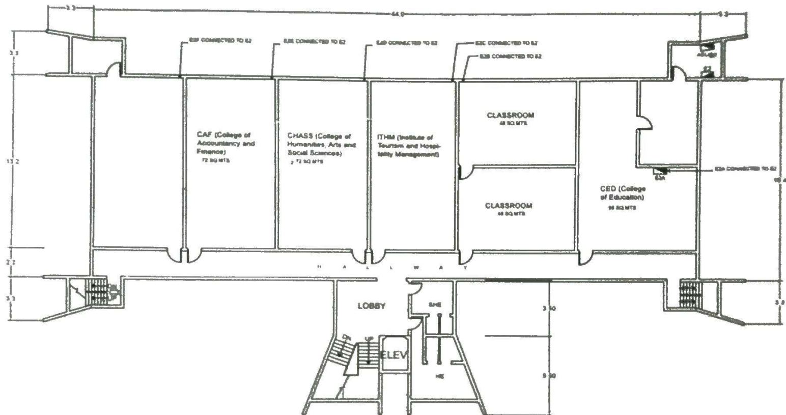
SECOND FLOOR POWER LAYOUT (GUSALING LACSON) SCALE: 1:100 METERS
