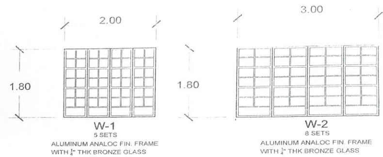
SCHEDULE OF WINDOWS SCALE NTS
